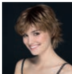
MIRANDA ** page 30
