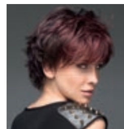
OPEN ** page 32
