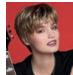
TOOL ** page 33
