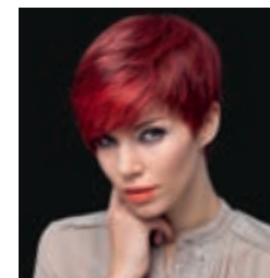
POINT ** page 27
